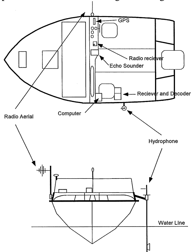
Figure 4 Equipment setup on a 6 m vessel for tracking trawl-caught turtles
